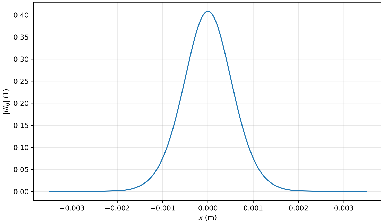
Intensity profile I(x, y = 0, z = 3.423m)/I_0 , P_{in}=0.4P_{cr} , artificial time
